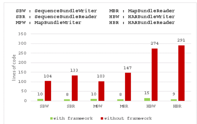
Fig. 10. Comparing file writers and readers with and without using framework
