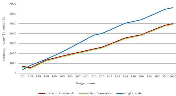
Fig. 7. Canny edge detection computation executed on a single node and on a Hadoop cluster with and without using framework
