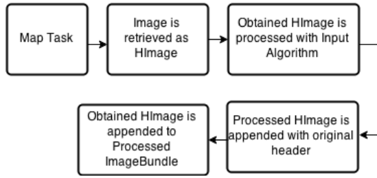
Fig. 3. Individual map task of Processor Module
