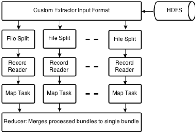
Fig. 6. Single node running the Extractor Module (handled by the framework and transparent to the user)
