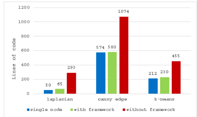
Fig. 9. Comparing coding complexity of Laplacian filter, Canny edge detection and k -means clustering in different environments
