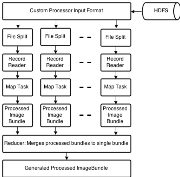
Fig. 4. Single node running the Processor Module (handled by the framework and transparent to user)
