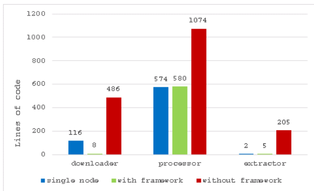
Fig. 8. Comparing coding complexities of modules in different environments
