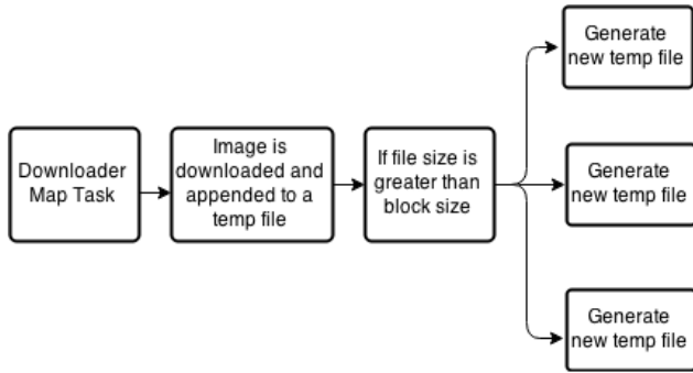
Fig. 1. Individual map task of Downloader Module
