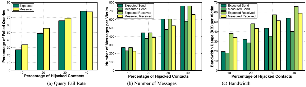
Figure 4: Large Scale Attack Simulation: 11, 303 ~ 16, 105 victims and 50 attackers. In (b) and (c) the numbers of messages and bandwidth costs are normalized based on the number of victims in each experiment.
